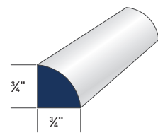
QUARTER ROUND AZM-105 LENGTH: 16'
