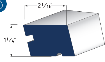
WINDOW SILL NOSE AZM-7974 LENGTH: 12'
